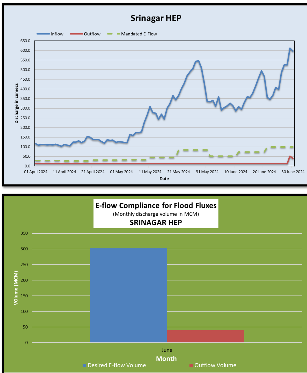
Figure 7: Graphs showing status of implementation of E-Flow at Srinagar HEP
