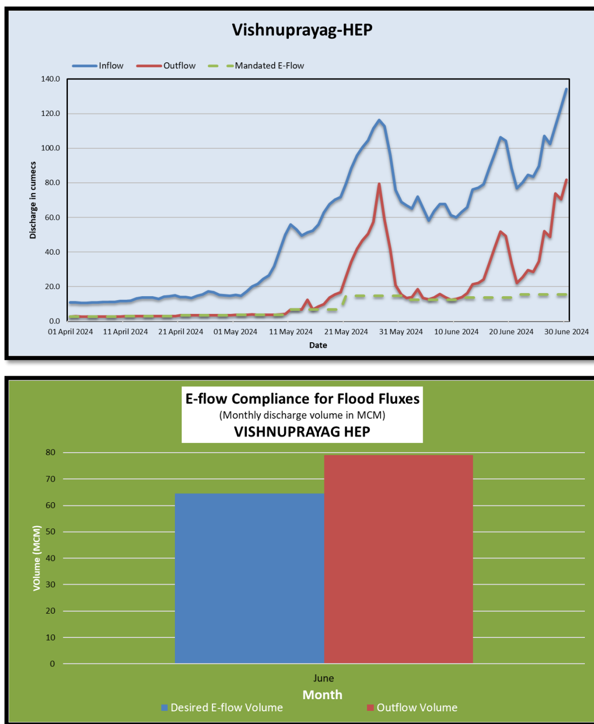
Figure 5: Graphs showing status of implementation of E-Flow at Vishnuprayag HEP
